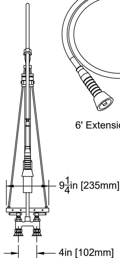
Quick Connect Coupler
